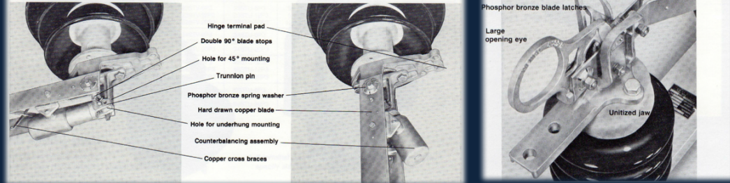
Hinge assembly arrangement of a closed, underhung mounted, switch complete with counterbalancing.
