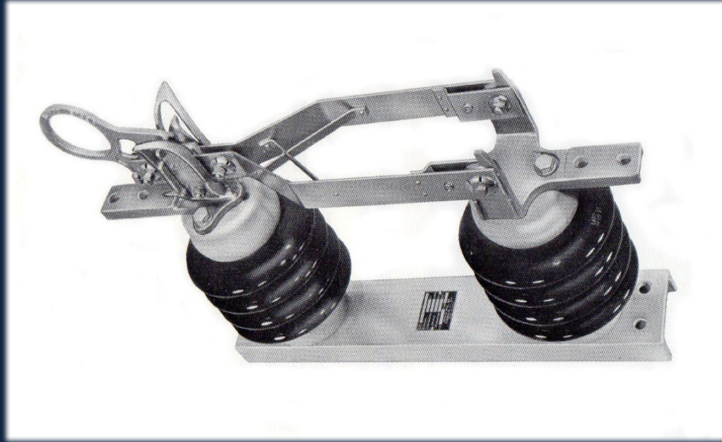
Hinge assembly arrangement of a closed, underhung mounted, switch complete with counterbalancing.
